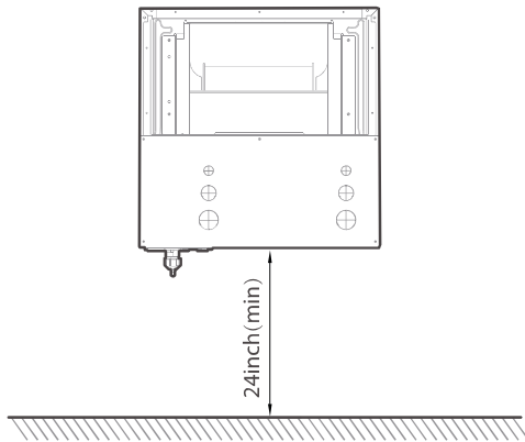
Vertical installations
