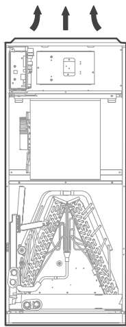
Upflow
