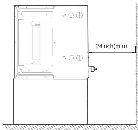
Installations horizontales
