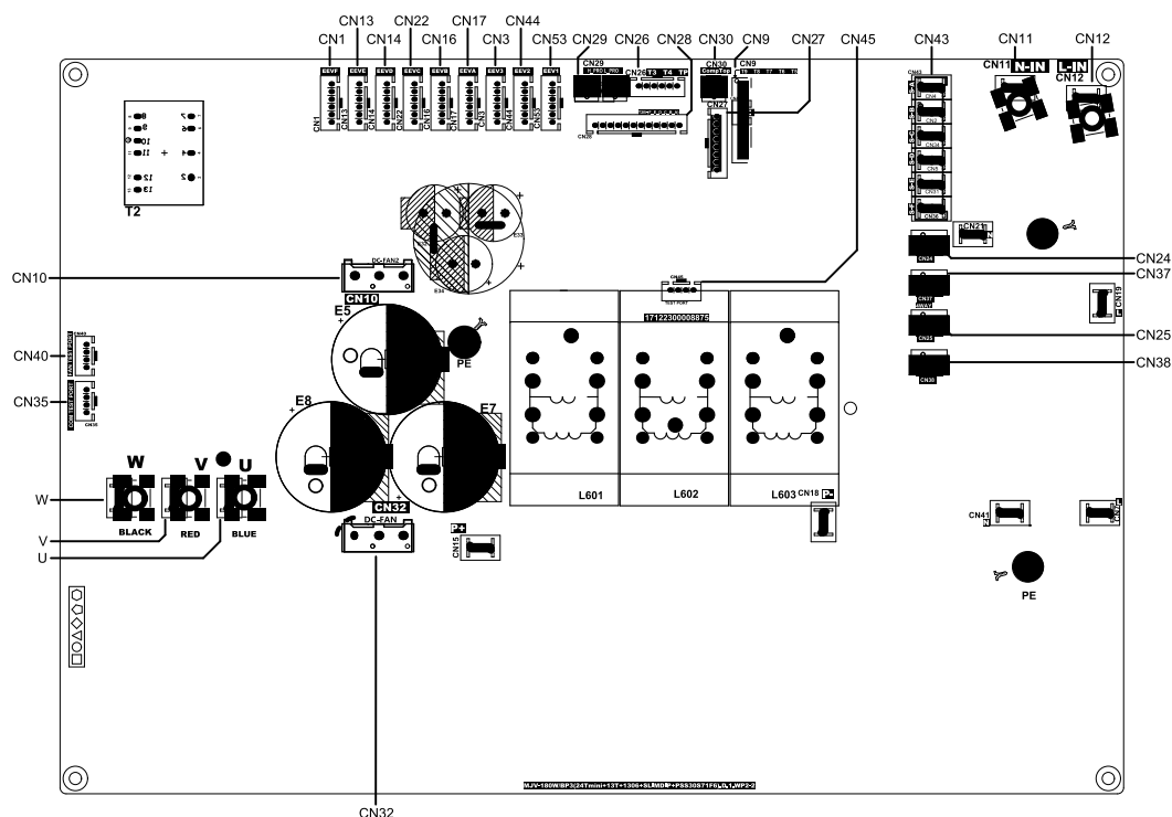
Outdoor unit printed circuit board diagram: 17122300008875
