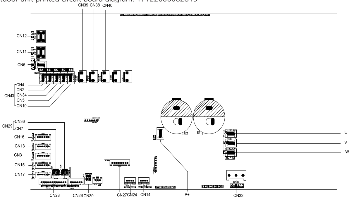
Outdoor unit printed circuit board diagram: 17122000062845
