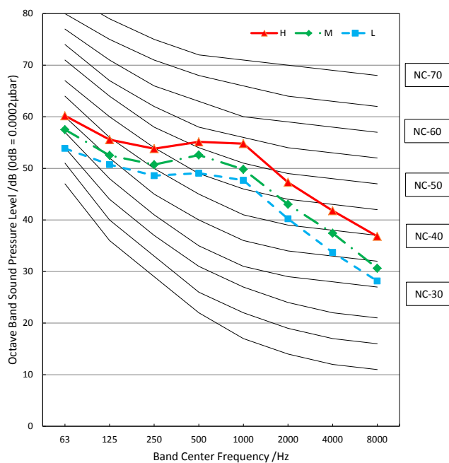
MHG-60HWFN1-MW
